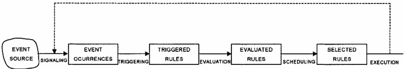
Figure 4. Rule execution [23]
