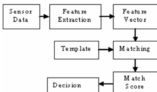
Figure 1. Biometric system [16]
